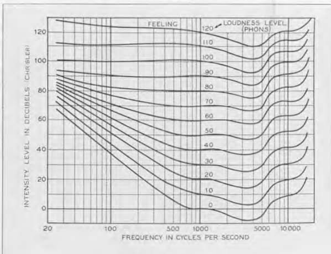
FIGURE 1. Equal-loudness contours for the average ear. 1
