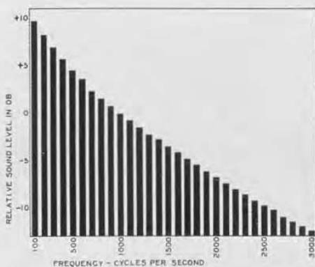
FIGURE 3. Chart of the relative contribution to total noise level made by 100-cycle bands over the frequency spectrum, as obtained from analyses of noises of a general character. (From A.S.A. Bulletin Z24.3 — 1936.)
