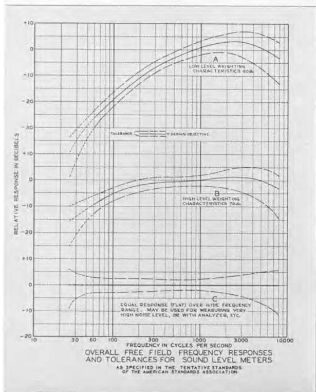
FIGURE 2. Design objective frequency-response curves between 60 and 8000 cycles for sound-level meters as specified by the American Standards Association (Bulletin Z24.3—1936). These standards do not specify the response below 60 cycles. The extended curves represent present practice as followed by the General Radio Company in the TYPE 759-B Sound-Level Meter.
